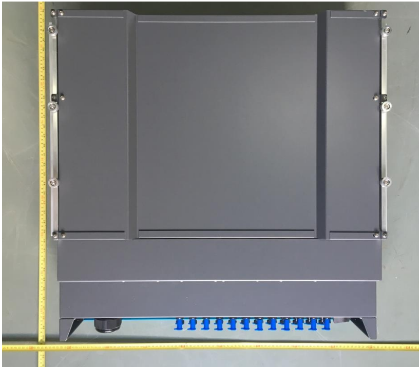
Back view
