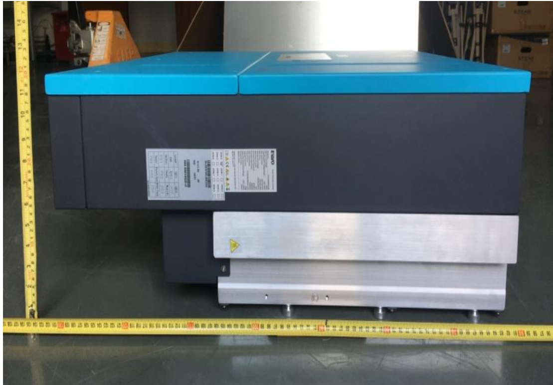
Side view
